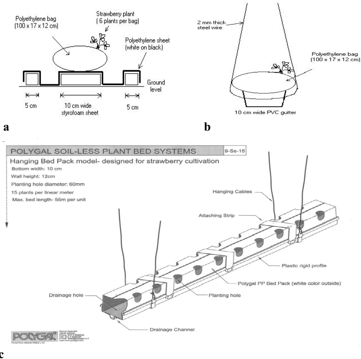
Fig. 1. (a) “Bag on ground” culture; (b) “Bag on gutter” culture; (c) Polygal® “Hanging Bed-Pack” trough. Printed with permission from Gilad Roter, Polygal, Israel.
